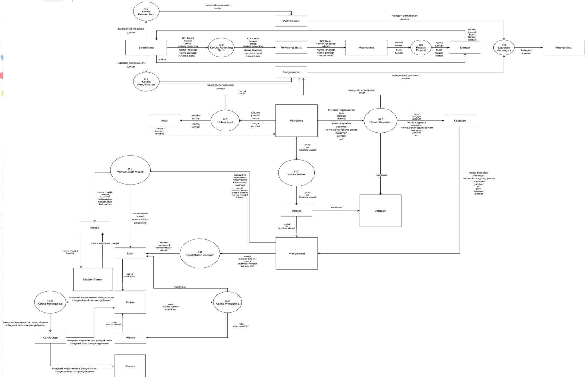
Gambar 14. Data Flow Diagram Level 0
