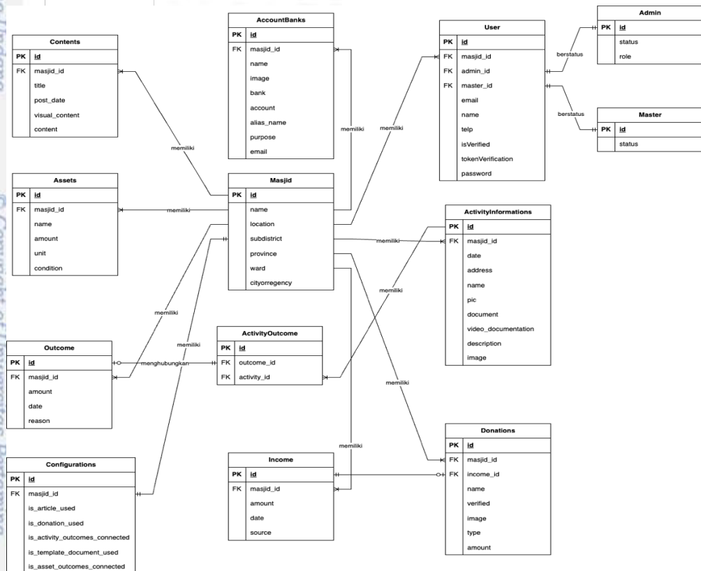
Gambar 12. Entity Relational Diagram Crow's Foot
