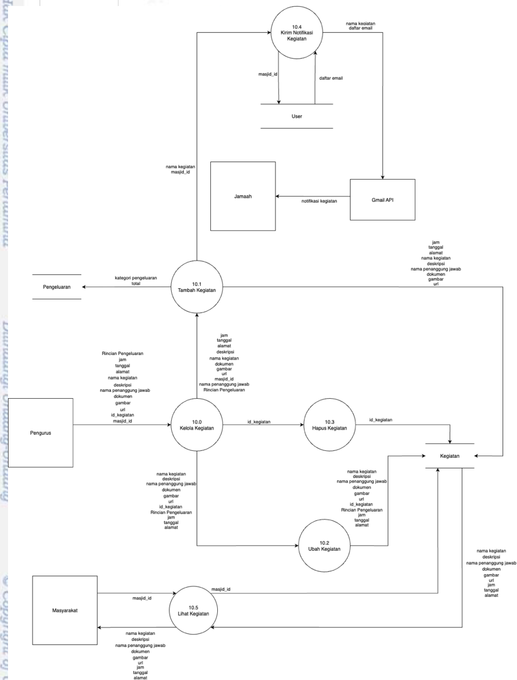
Gambar 19. Data Flow Diagram Level 1 – Kelola Kegiatan
